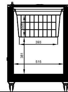
Section side
