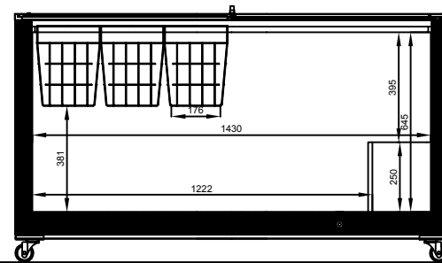
Section front
