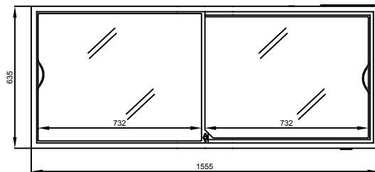
Top closed
