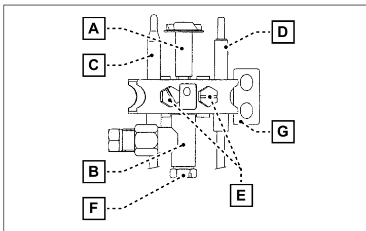
Fig. 21 Pilot nozzle main parts
