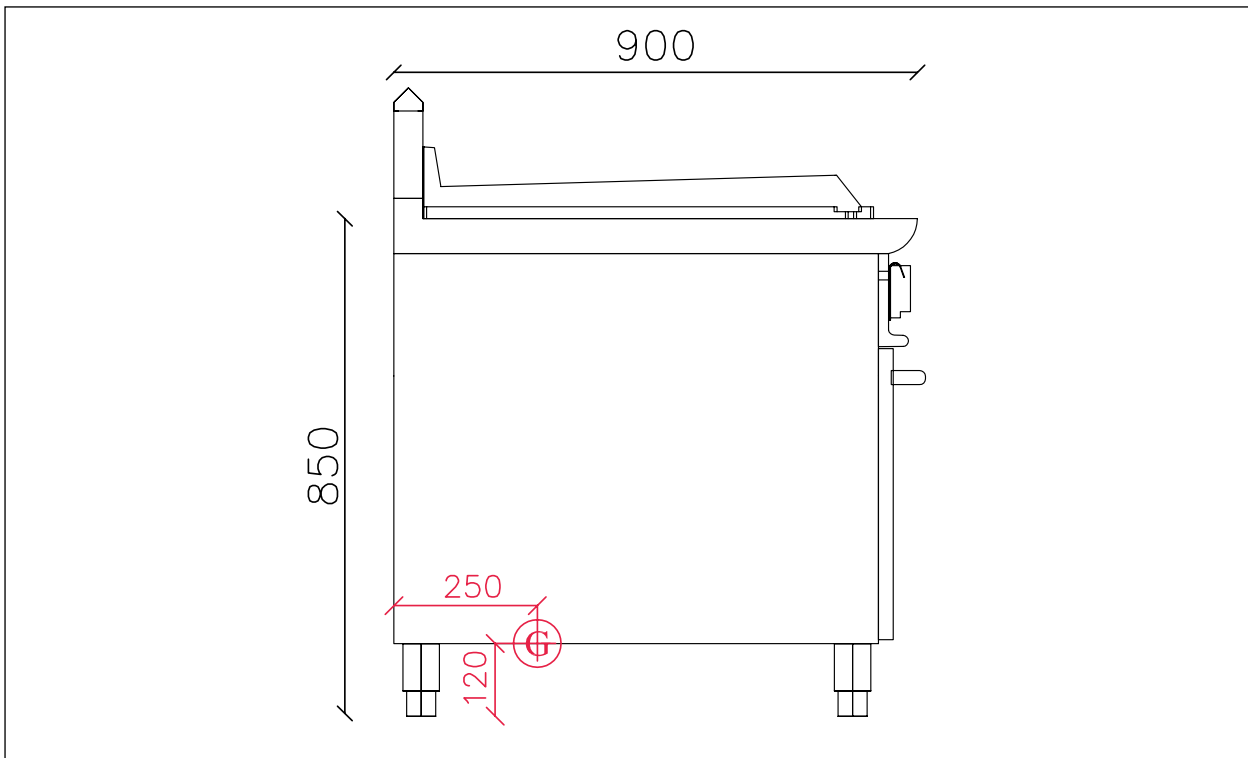
Fig. 9 Dimensions of griddle plate with cabinet
