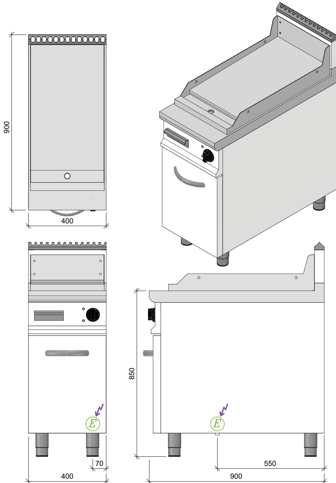
Fig. 12 Fry-top with closed stand and small plate size
