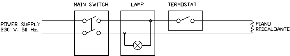
Fig.n.5 - Single phase electrical layout 230V/50Hz - on mod.C
