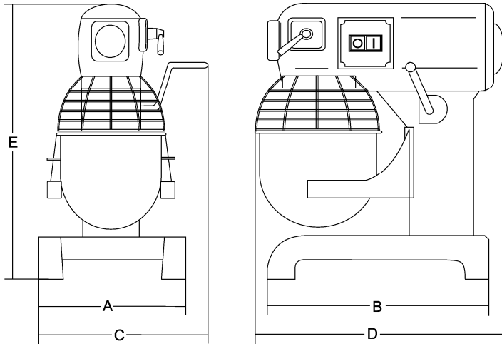
FIG. n.2 - Overall dimensions
